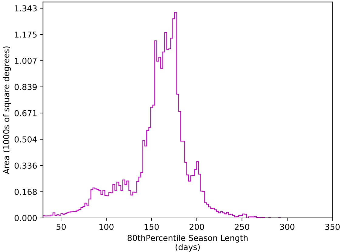
too_elab_r16_d3_giz_v3.4_10yrs All sky z band: 80thPercentile Season Length
