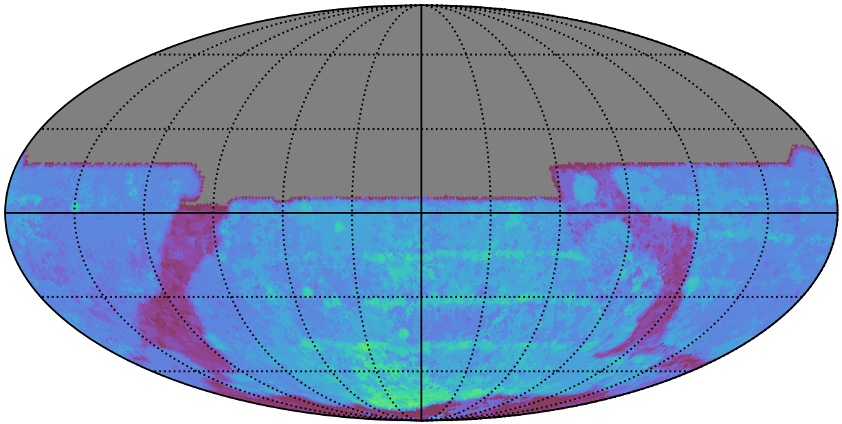
too_elab_r16_d3_giz_v3.4_10yrs All sky y band: 80thPercentile Season Length
