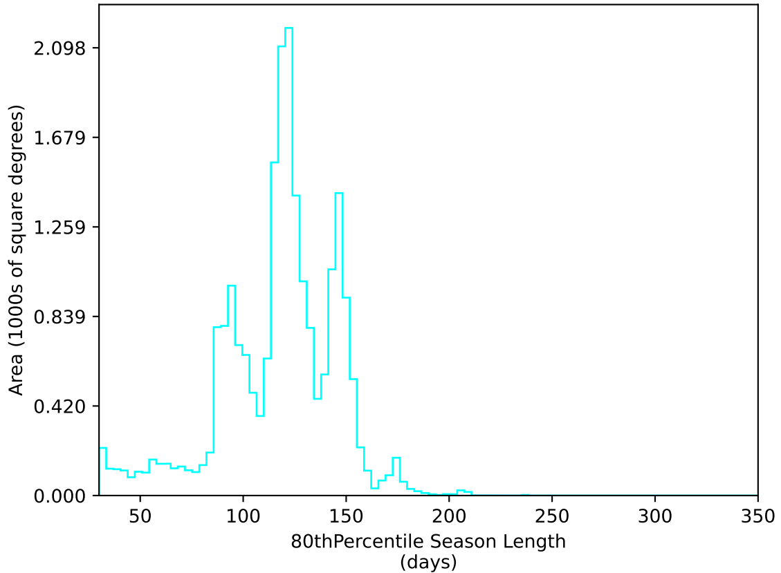
too_elab_r16_d3_giz_v3.4_10yrs All sky u band: 80thPercentile Season Length
