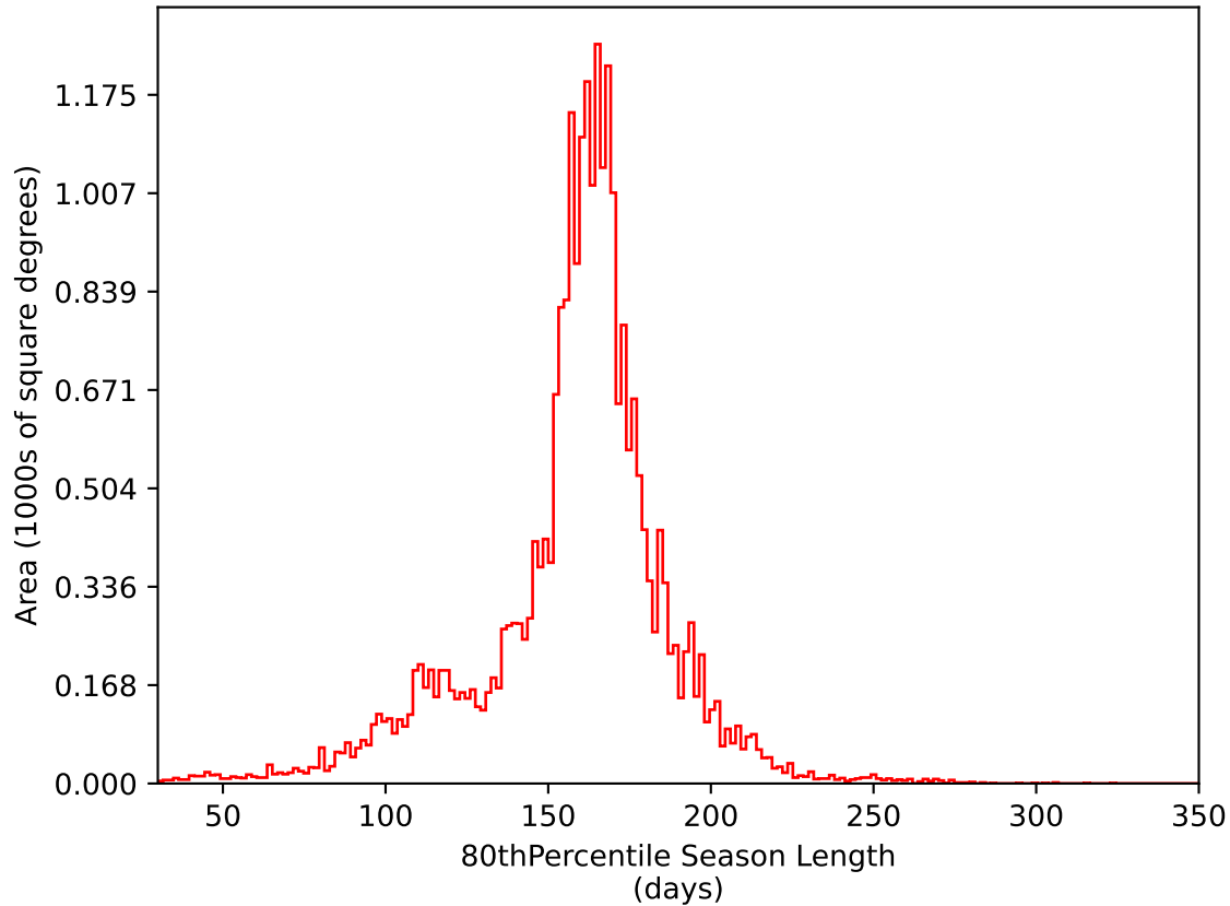
too_elab_r16_d3_giz_v3.4_10yrs All sky i band: 80thPercentile Season Length
