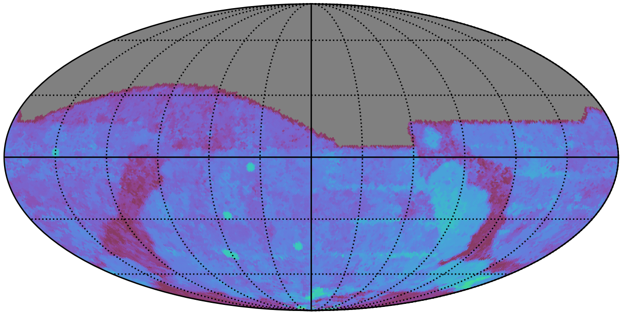
too_elab_r16_d3_giz_v3.4_10yrs All sky g band: 80thPercentile Season Length
