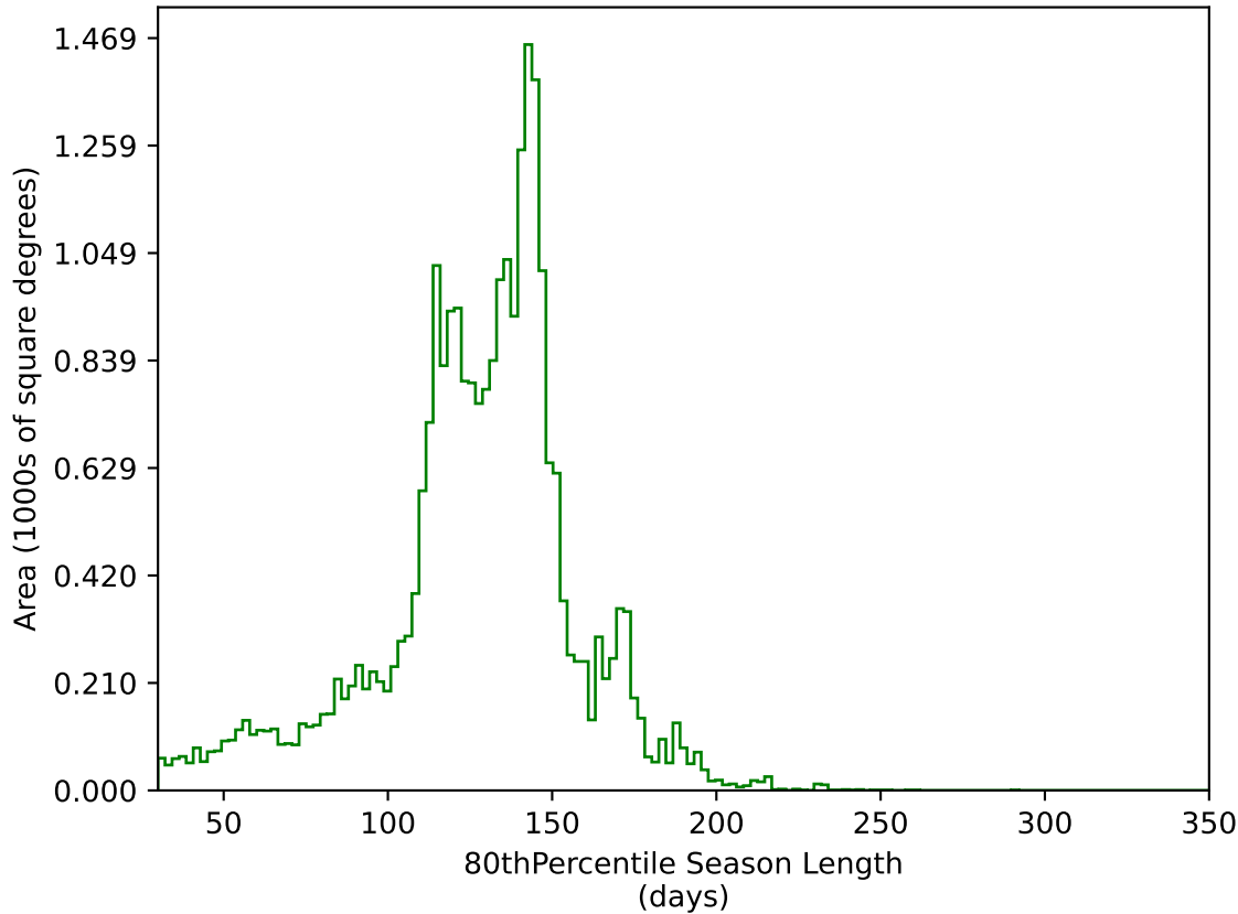
too_elab_r16_d3_giz_v3.4_10yrs All sky g band: 80thPercentile Season Length
