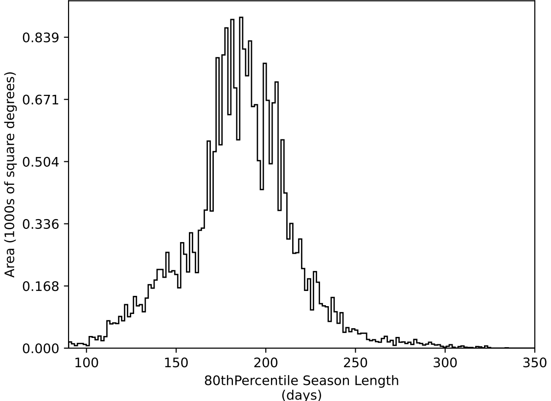
too_elab_r16_d3_giz_v3.4_10yrs All sky all bands: 80thPercentile Season Length
