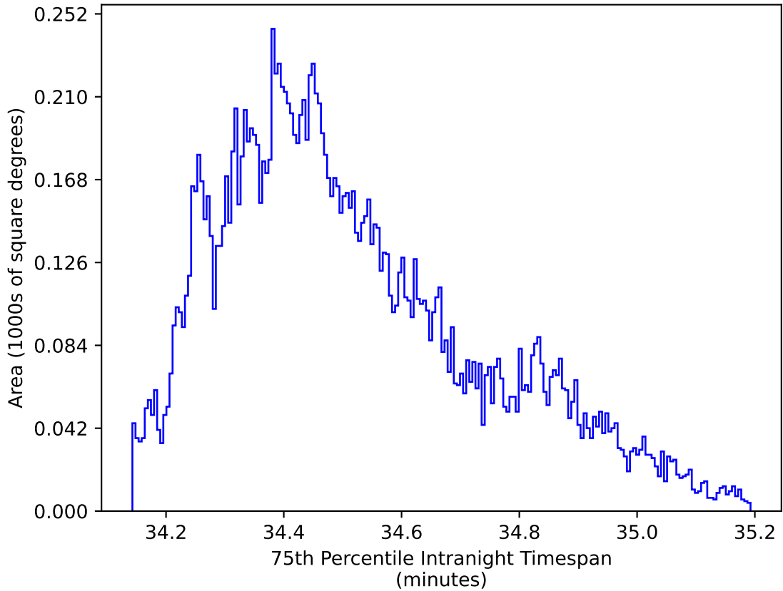
too_elab_r16_d3_giz_v3.4_10yrs WFD zy bands: 75th Percentile Intranight Timespan
