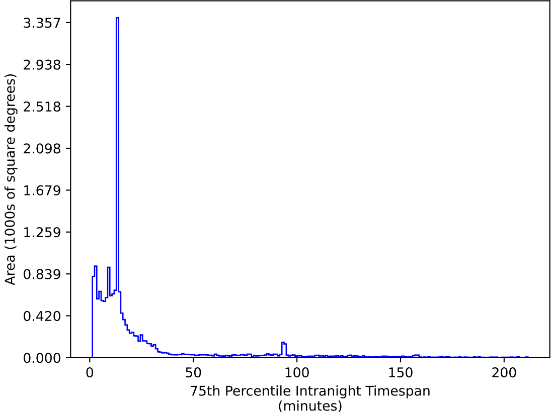
too_elab_r16_d3_giz_v3.4_10yrs WFD z band: 75th Percentile Intranight Timespan
