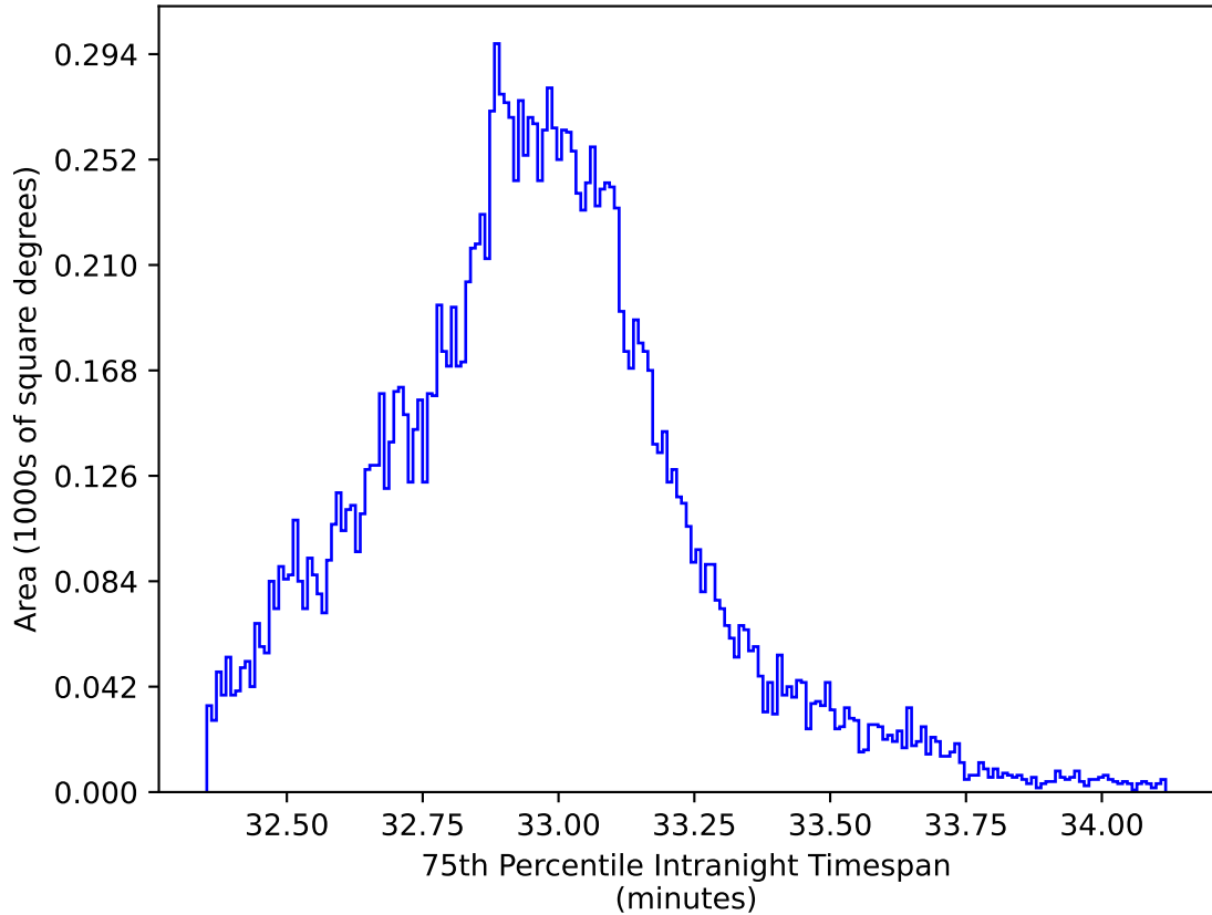
too_elab_r16_d3_giz_v3.4_10yrs WFD y band: 75th Percentile Intranight Timespan
