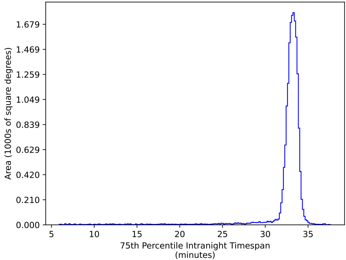
too_elab_r16_d3_giz_v3.4_10yrs WFD ug bands: 75th Percentile Intranight Timespan
