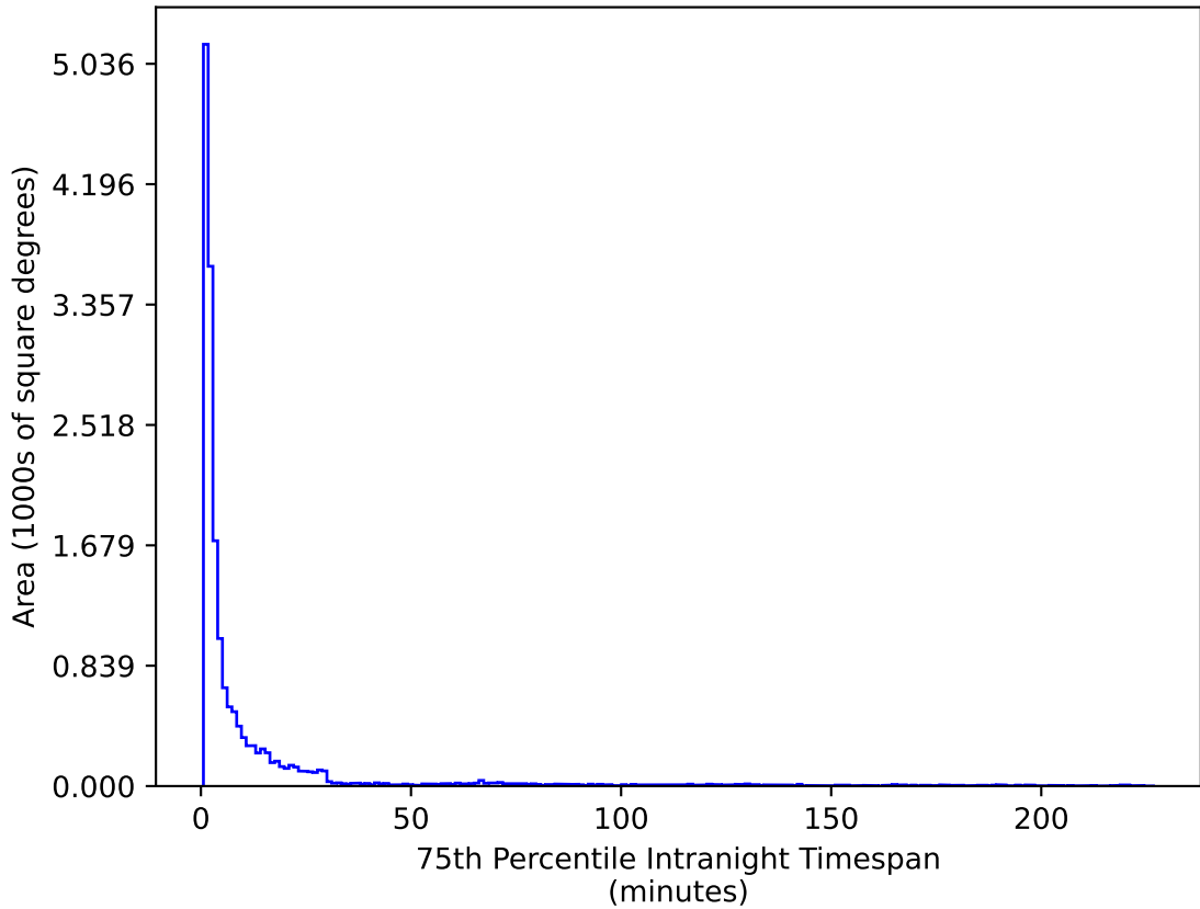
too_elab_r16_d3_giz_v3.4_10yrs WFD u band: 75th Percentile Intranight Timespan
