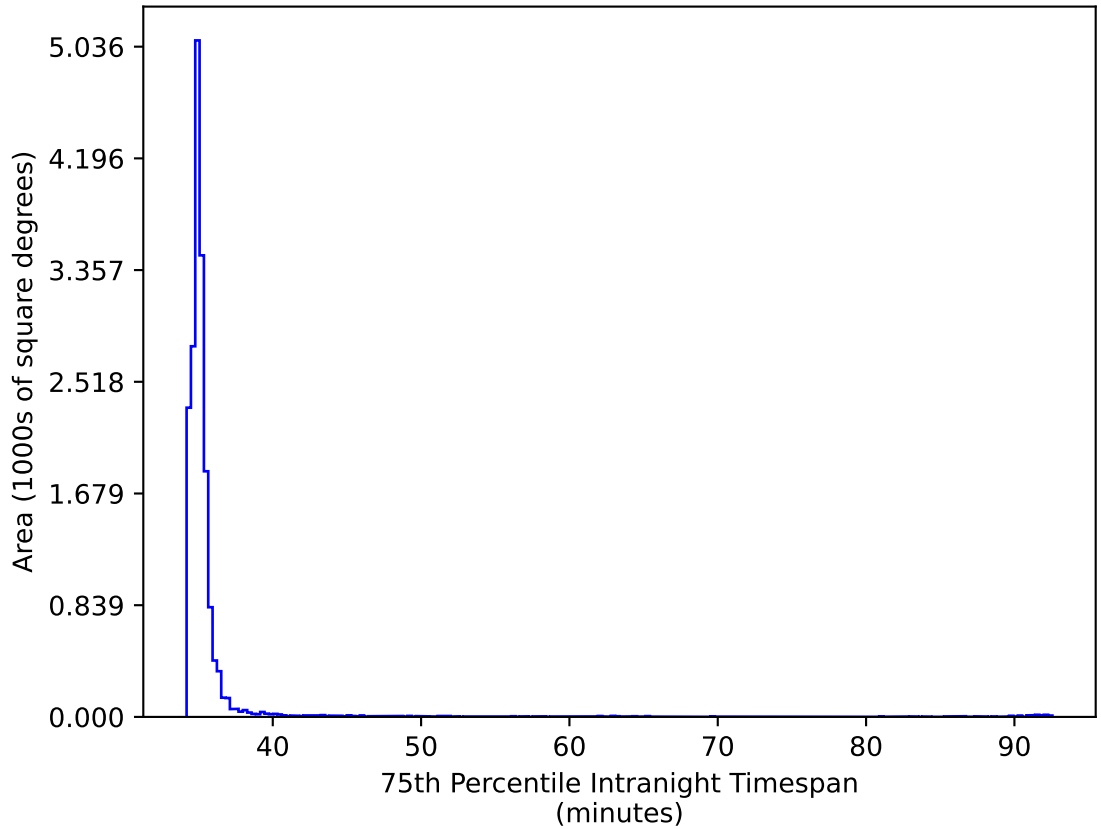
too_elab_r16_d3_giz_v3.4_10yrs WFD ri bands: 75th Percentile Intranight Timespan
