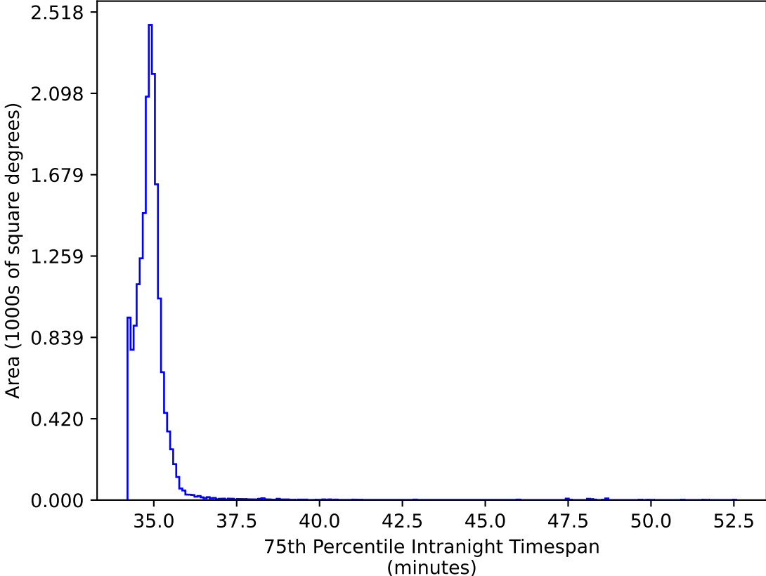
too_elab_r16_d3_giz_v3.4_10yrs WFD iz bands: 75th Percentile Intranight Timespan
