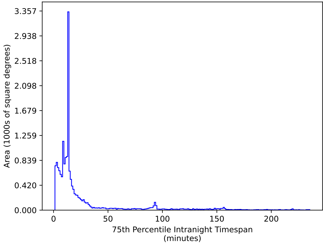
too_elab_r16_d3_giz_v3.4_10yrs WFD i band: 75th Percentile Intranight Timespan
