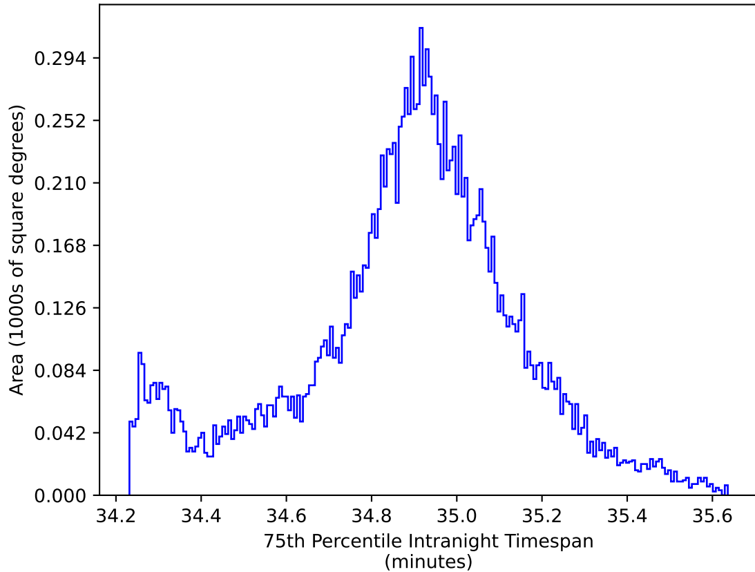
too_elab_r16_d3_giz_v3.4_10yrs WFD all bands: 75th Percentile Intranight Timespan
