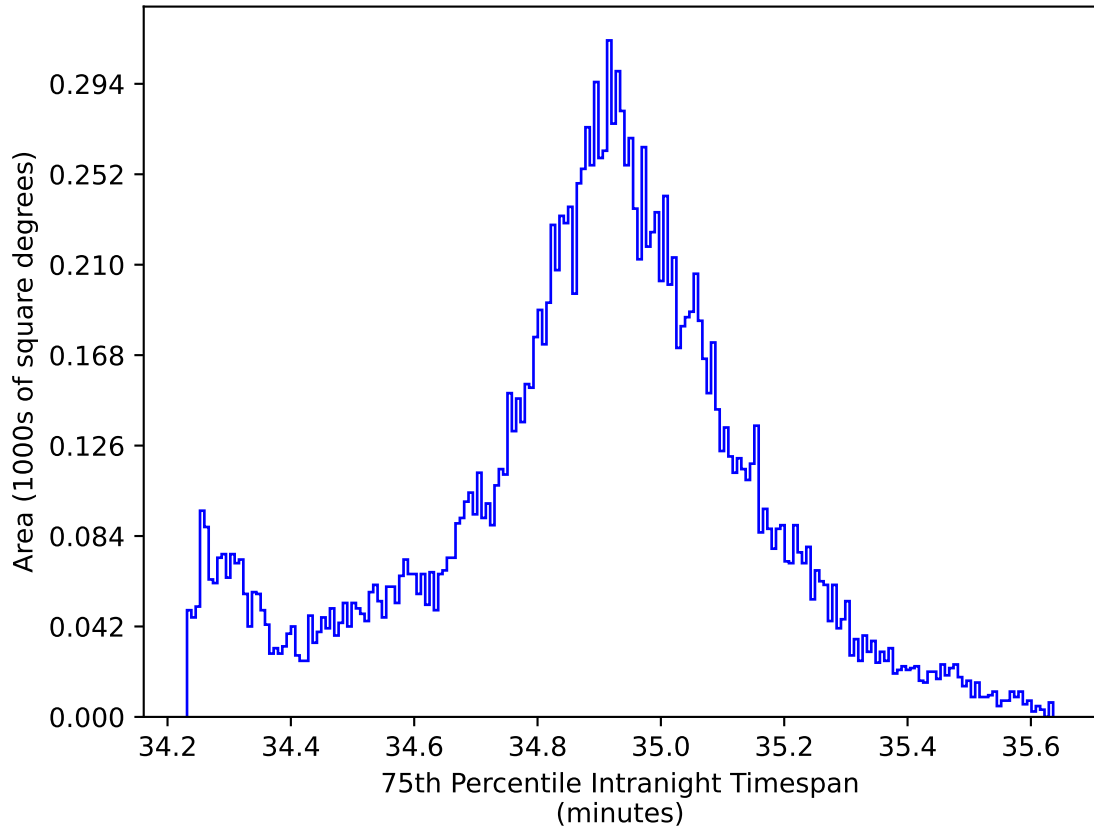
too_elab_r16_d3_giz_v3.4_10yrs WFD: 75th Percentile Intranight Timespan
