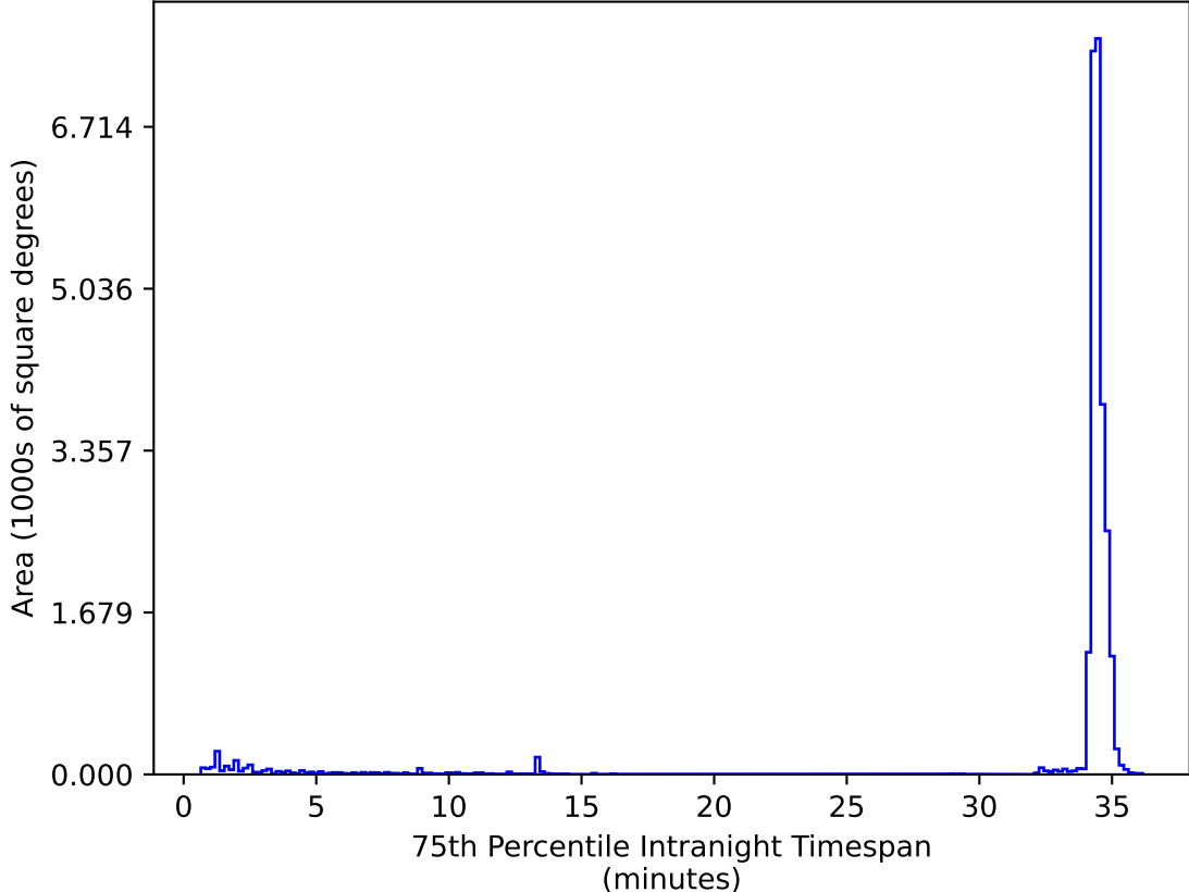
too_elab_r16_d3_giz_v3.4_10yrs All sky zy bands: 75th Percentile Intranight Timespan
