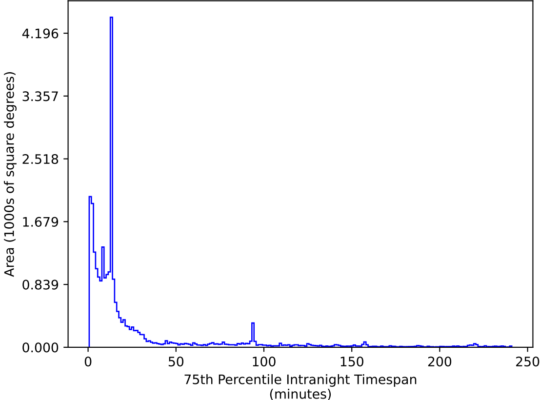
too_elab_r16_d3_giz_v3.4_10yrs All sky z band: 75th Percentile Intranight Timespan
