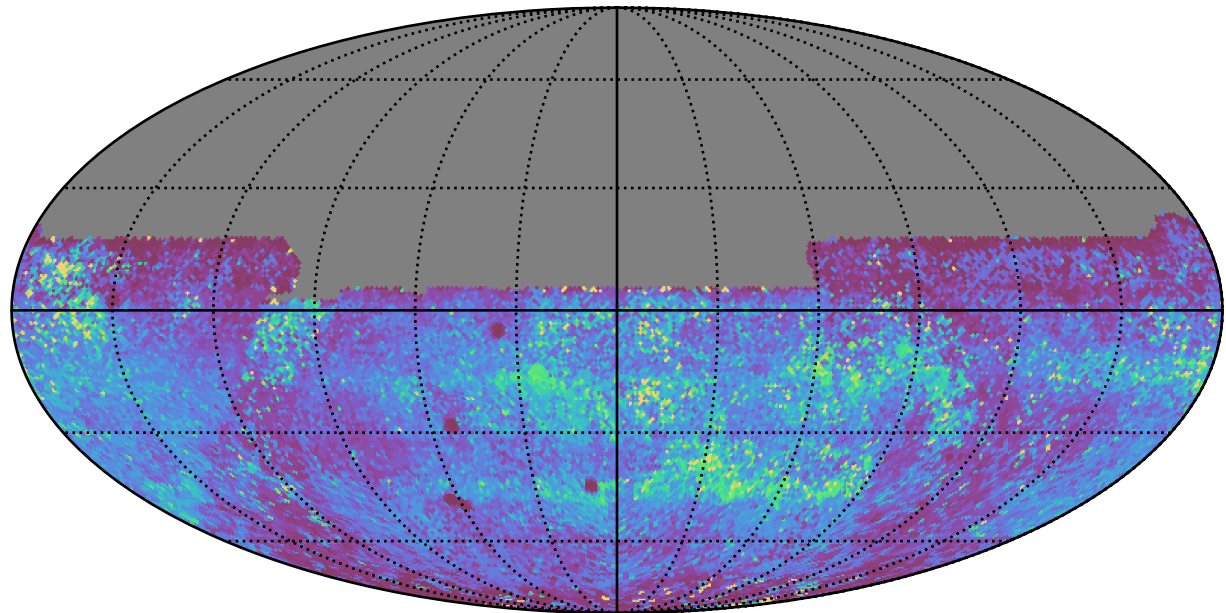
too_elab_r16_d3_giz_v3.4_10yrs All sky y band: 75th Percentile Intranight Timespan
