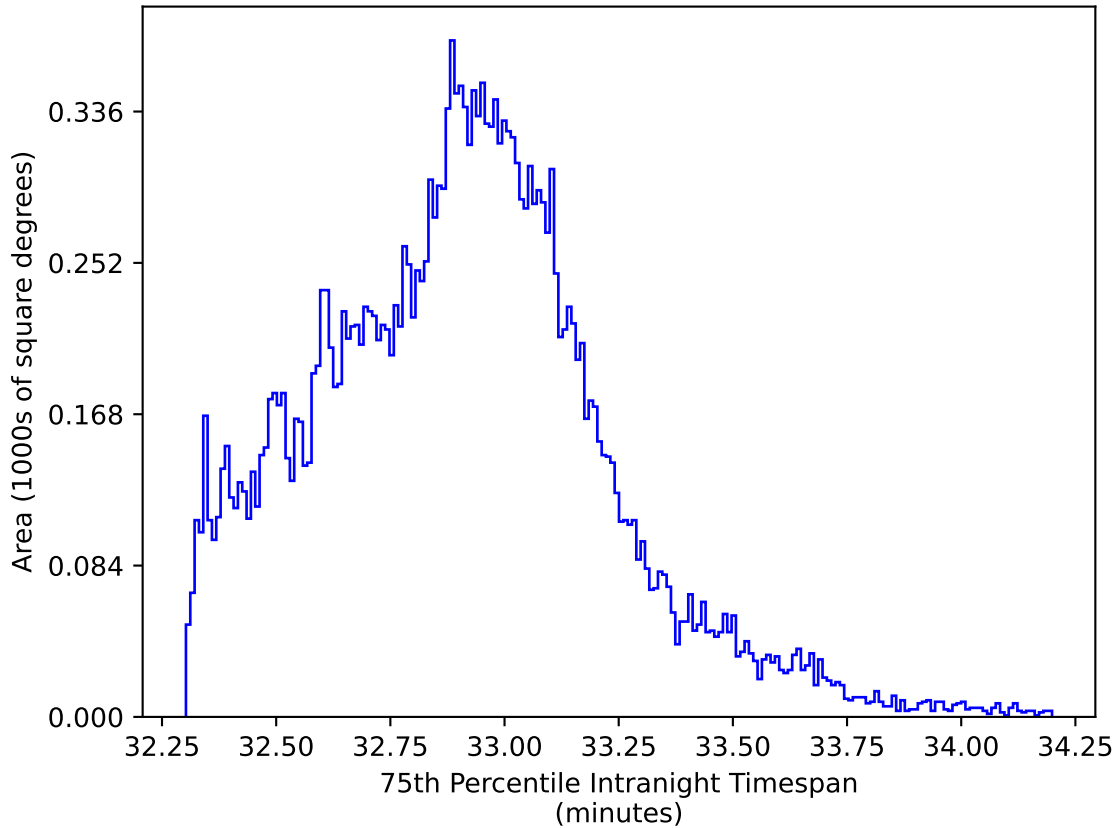
too_elab_r16_d3_giz_v3.4_10yrs All sky y band: 75th Percentile Intranight Timespan
