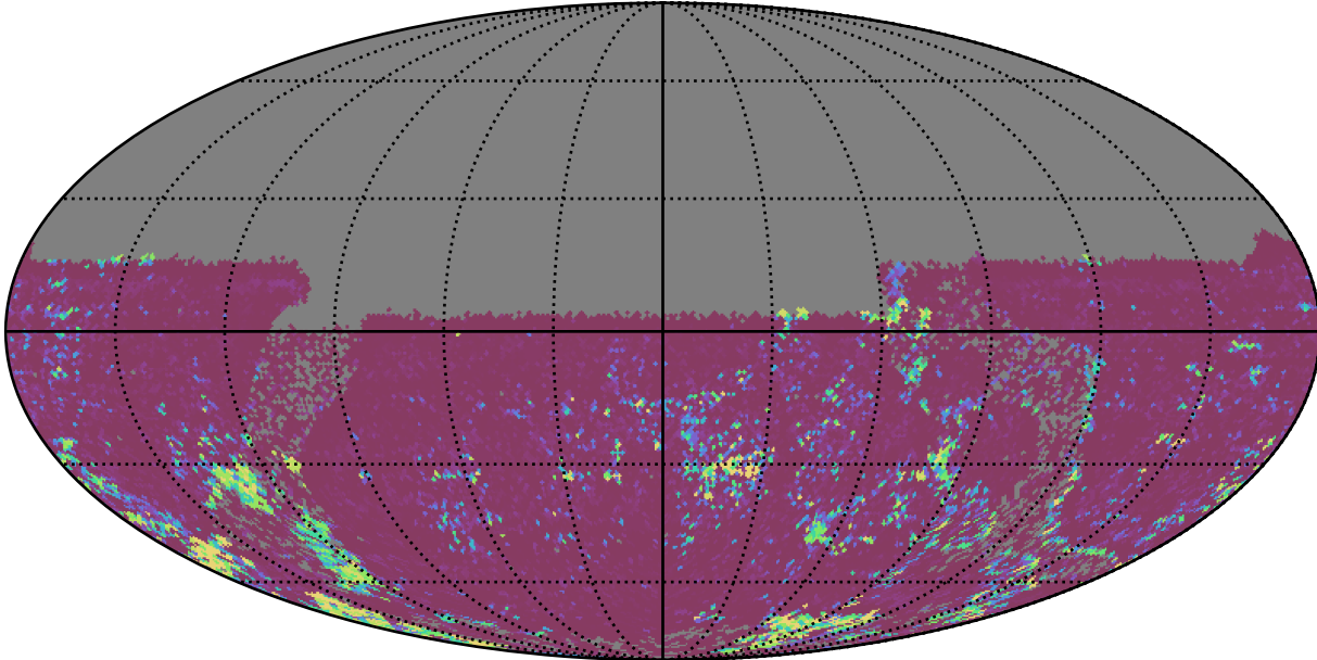
too_elab_r16_d3_giz_v3.4_10yrs All sky u band: 75th Percentile Intranight Timespan
