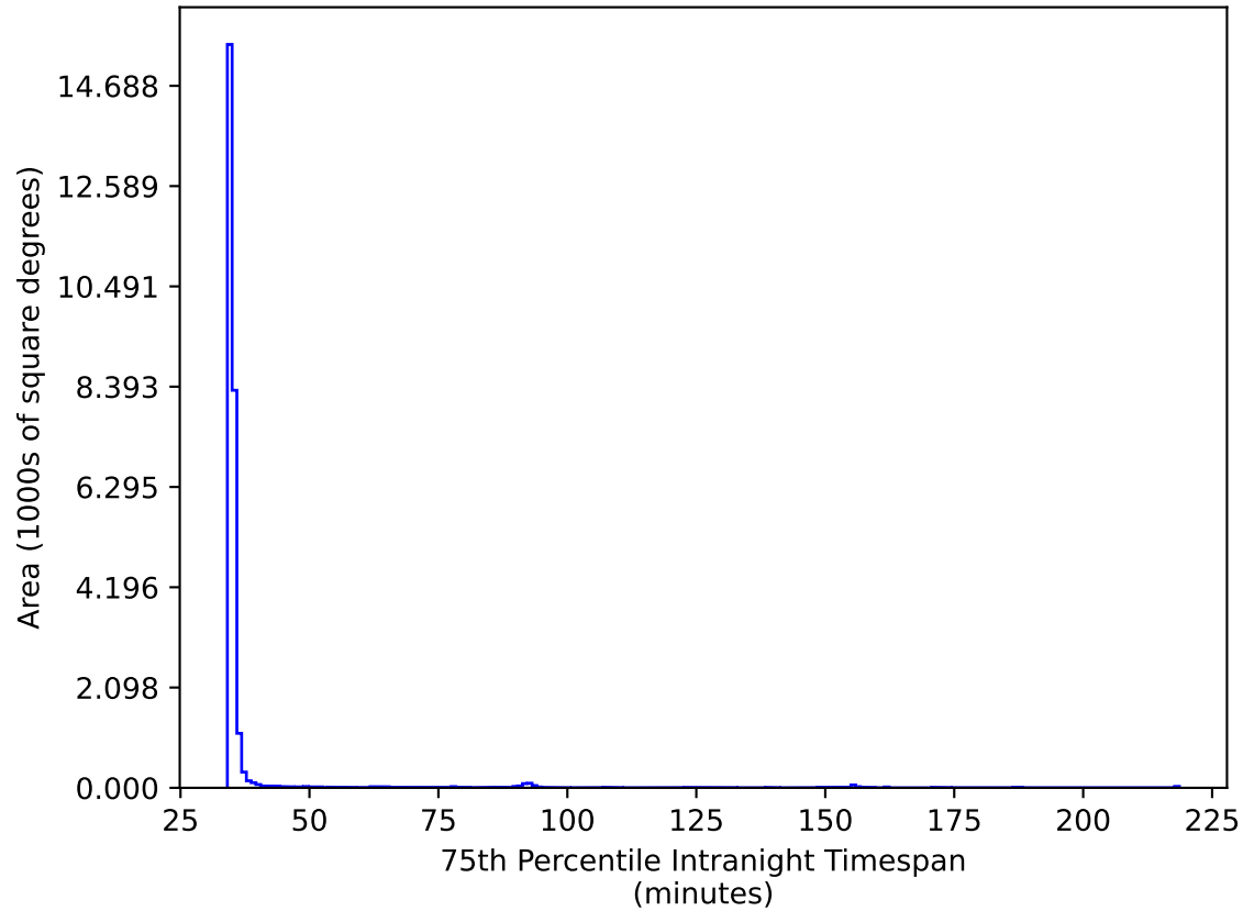
too_elab_r16_d3_giz_v3.4_10yrs All sky ri bands: 75th Percentile Intranight Timespan
