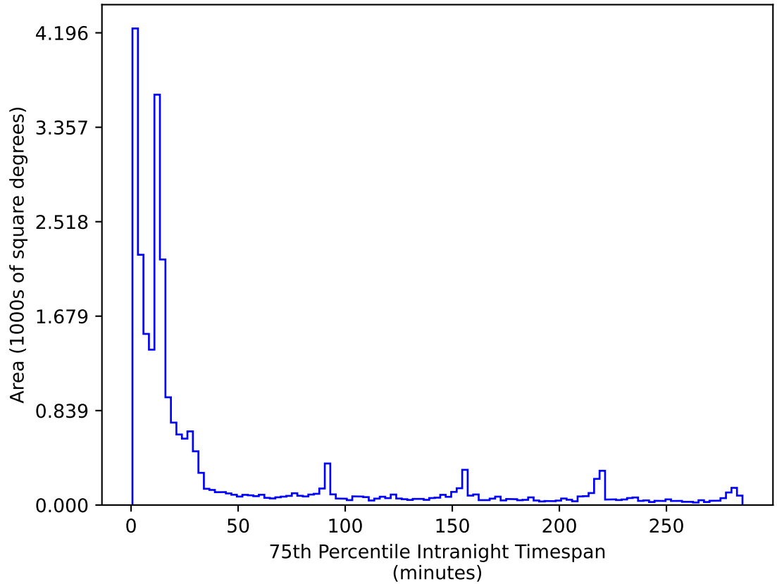
too_elab_r16_d3_giz_v3.4_10yrs All sky r band: 75th Percentile Intranight Timespan
