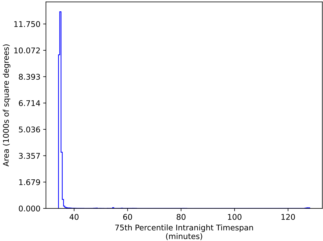
too_elab_r16_d3_giz_v3.4_10yrs All sky iz bands: 75th Percentile Intranight Timespan
