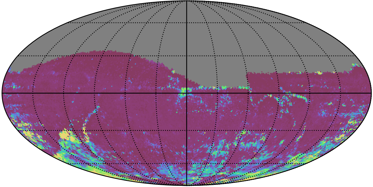
too_elab_r16_d3_giz_v3.4_10yrs All sky i band: 75th Percentile Intranight Timespan
