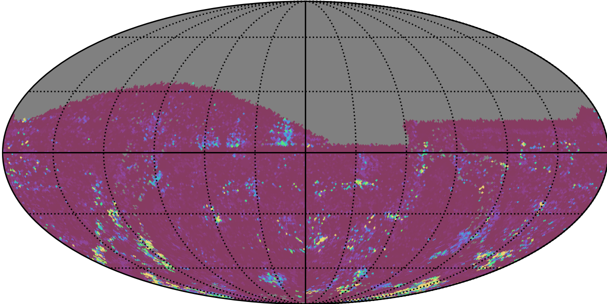
too_elab_r16_d3_giz_v3.4_10yrs All sky g band: 75th Percentile Intranight Timespan
