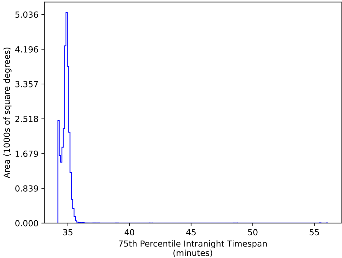
too_elab_r16_d3_giz_v3.4_10yrs All sky: 75th Percentile Intranight Timespan
