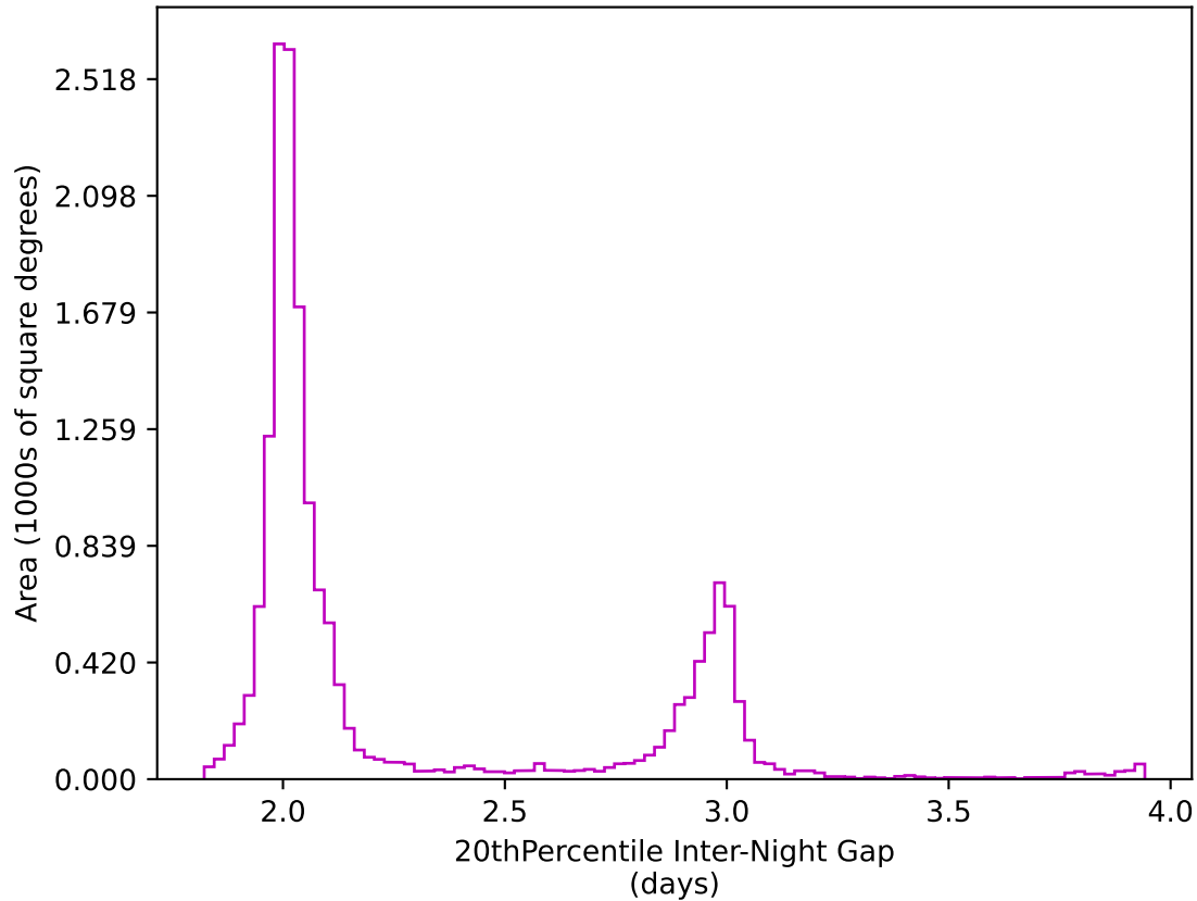
too_elab_r16_d3_giz_v3.4_10yrs WFD z band: 20thPercentile Inter-Night Gap
