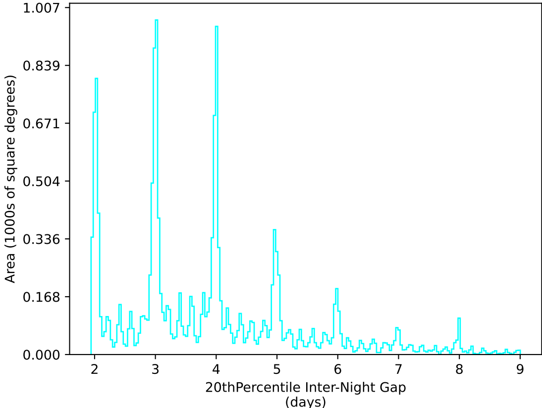
too_elab_r16_d3_giz_v3.4_10yrs WFD u band: 20thPercentile Inter-Night Gap
