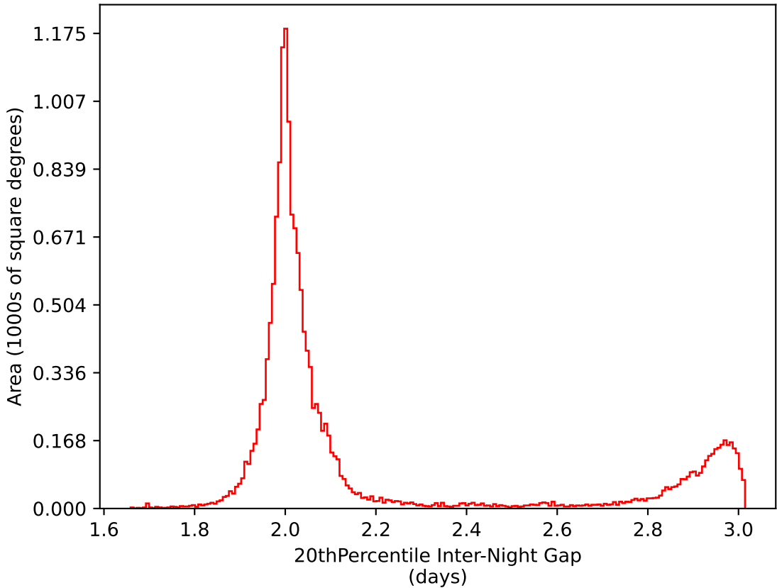
too_elab_r16_d3_giz_v3.4_10yrs WFD i band: 20thPercentile Inter-Night Gap
