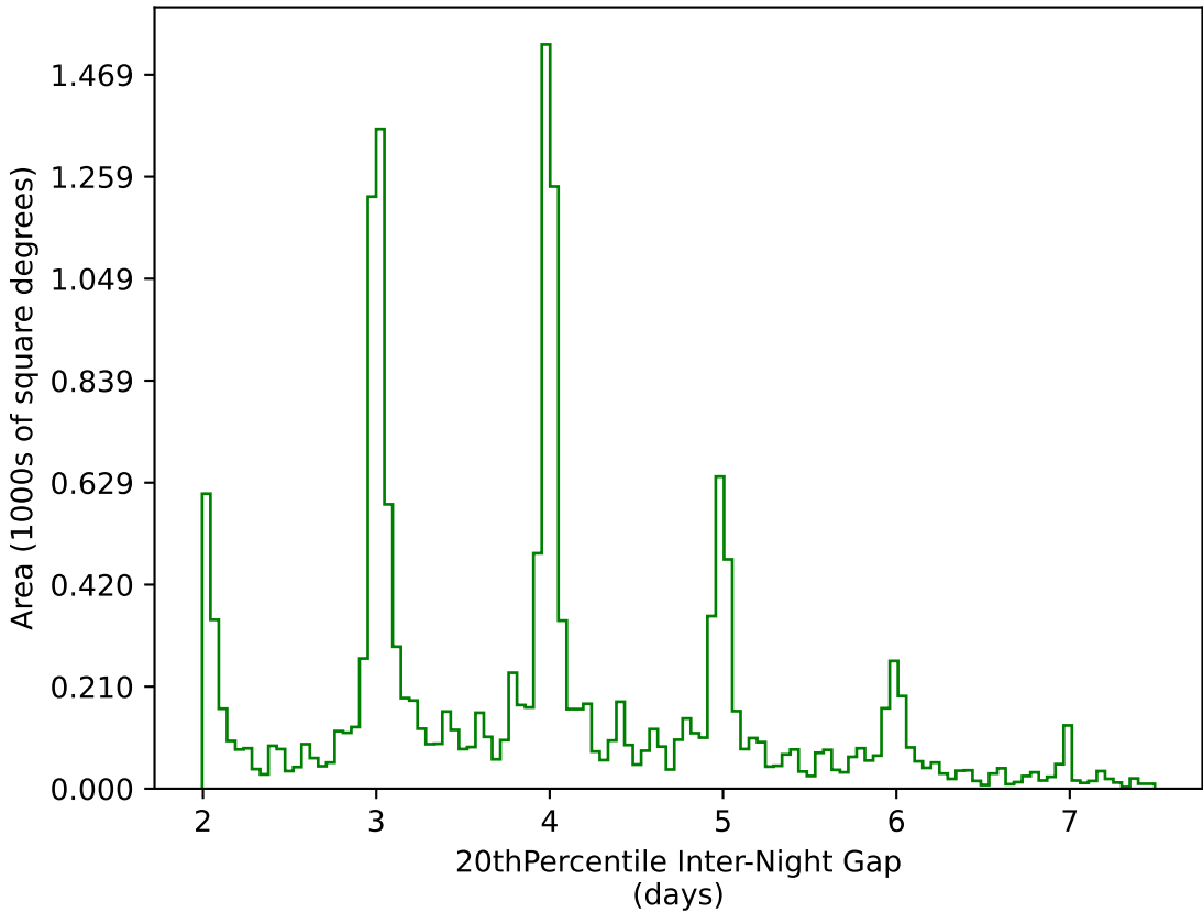
too_elab_r16_d3_giz_v3.4_10yrs WFD g band: 20thPercentile Inter-Night Gap
