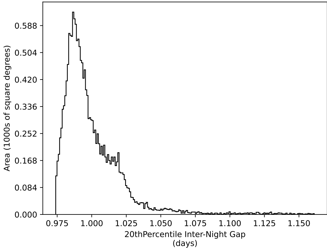
too_elab_r16_d3_giz_v3.4_10yrs WFD all bands: 20thPercentile Inter-Night Gap
