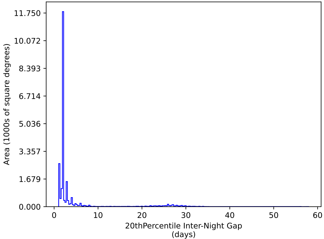
too_elab_r16_d3_giz_v3.4_10yrs All sky y band: 20thPercentile Inter-Night Gap
