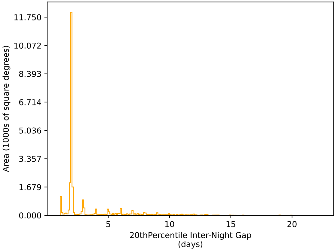
too_elab_r16_d3_giz_v3.4_10yrs All sky r band: 20thPercentile Inter-Night Gap
