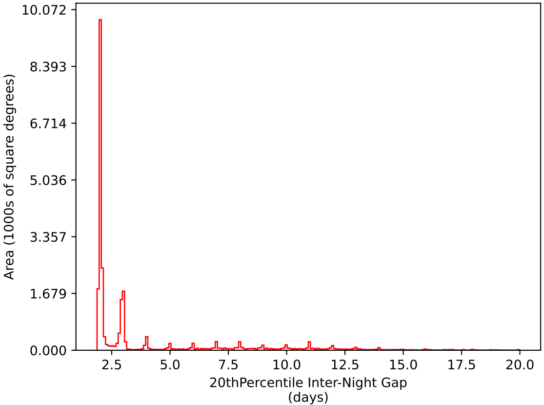
too_elab_r16_d3_giz_v3.4_10yrs All sky i band: 20thPercentile Inter-Night Gap
