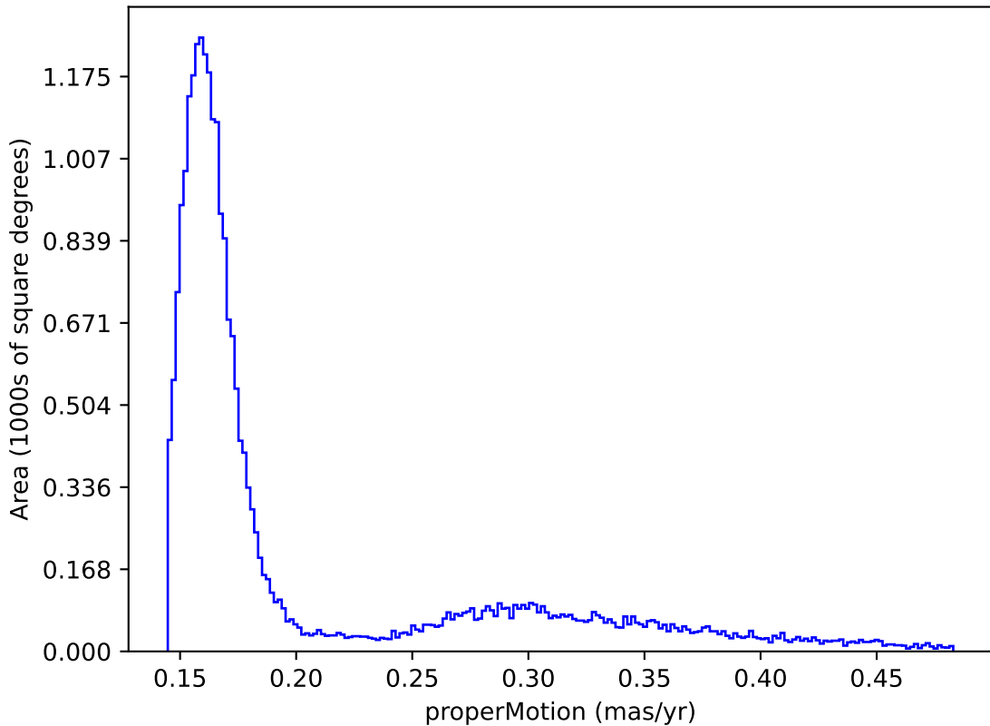
too_elab_r16_d3_giz_v3.4_10yrs : properMotion
