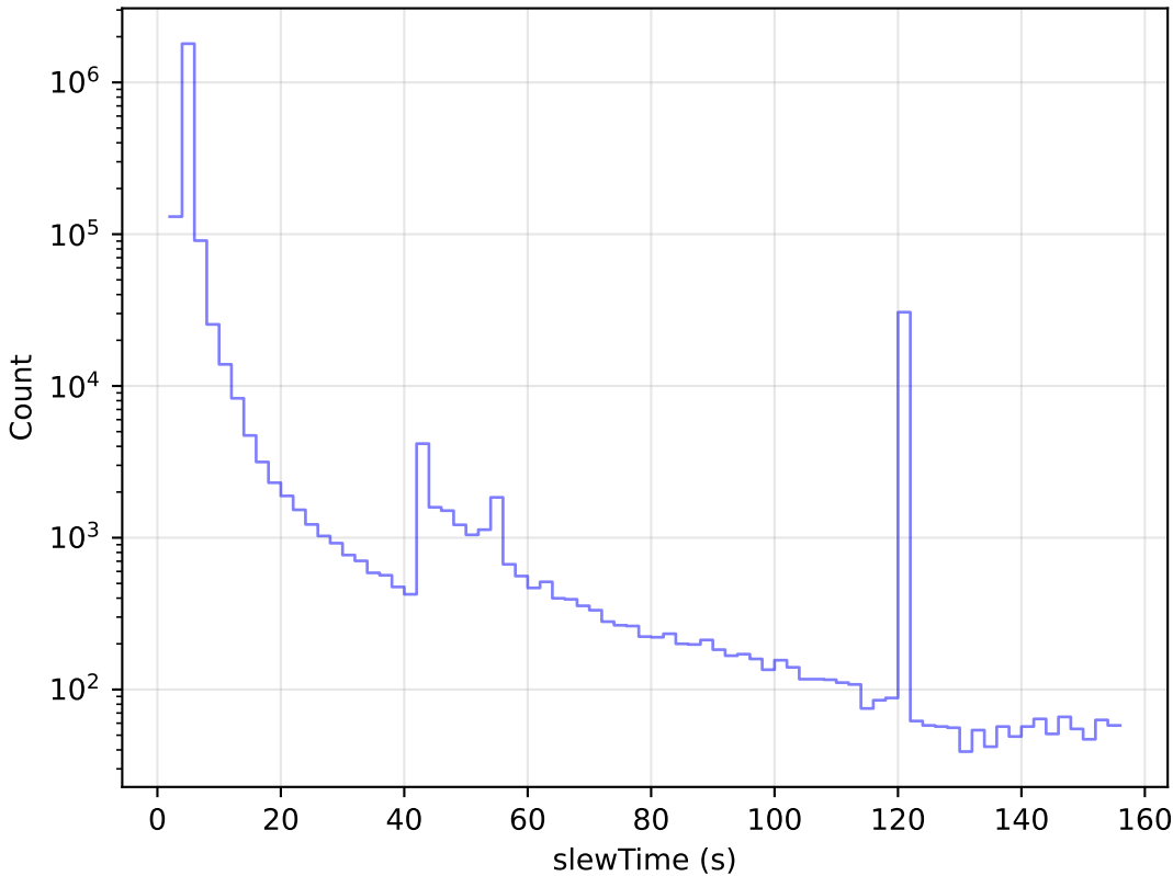
too_elab_r16_d3_giz_v3.4_10yrs All visits: Slew Time Histogram
