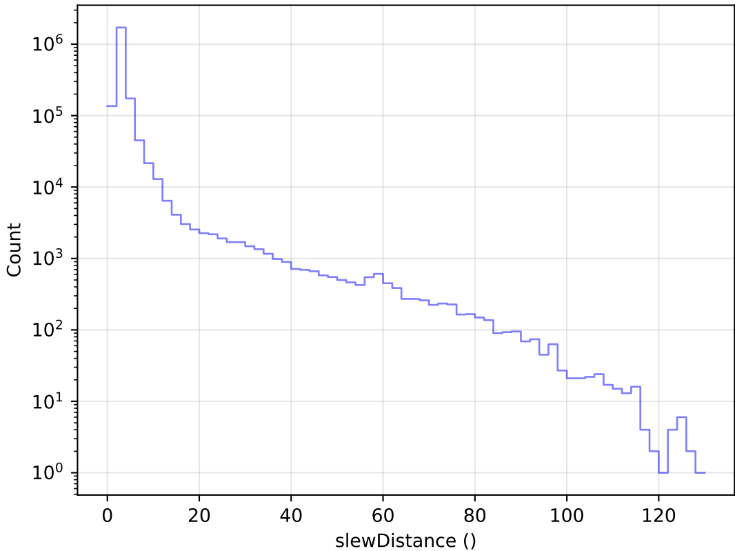
too_elab_r16_d3_giz_v3.4_10yrs All visits: Slew Distance Histogram
