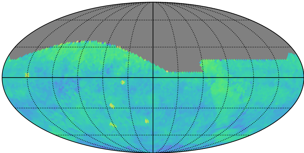
too_elab_r16_d3_giz_v3.4_10yrs (g or r or i): PairFraction
