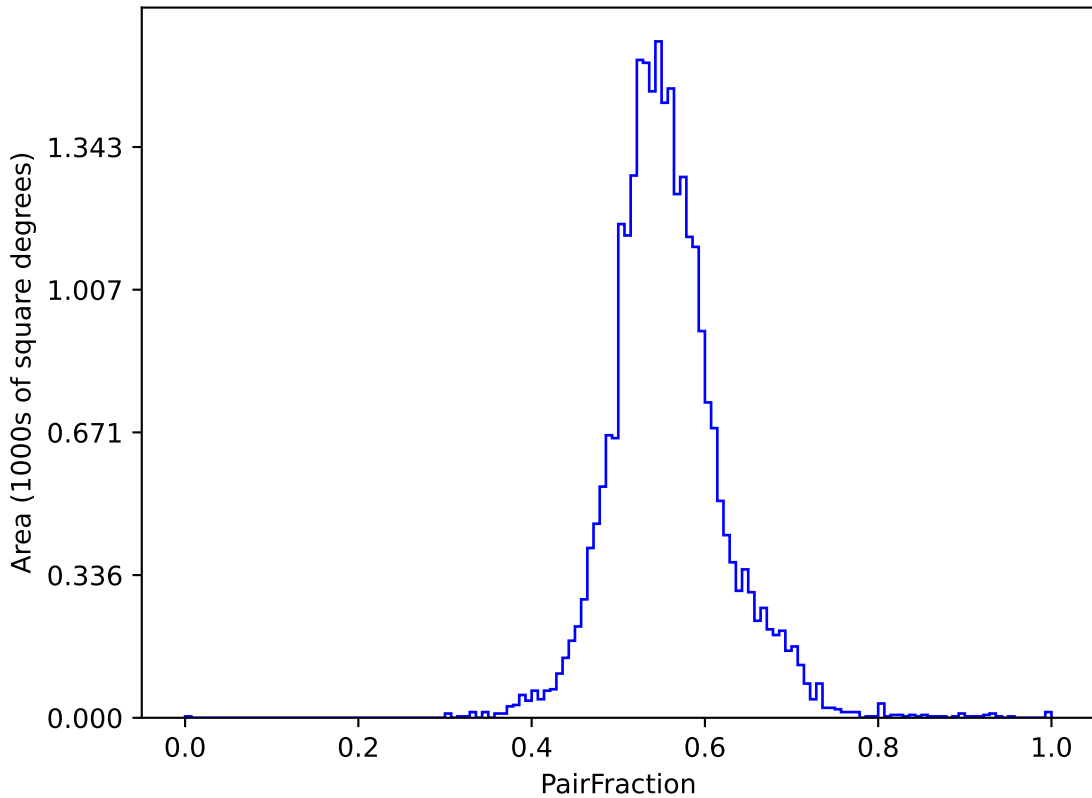
too_elab_r16_d3_giz_v3.4_10yrs (g or r or i): PairFraction
