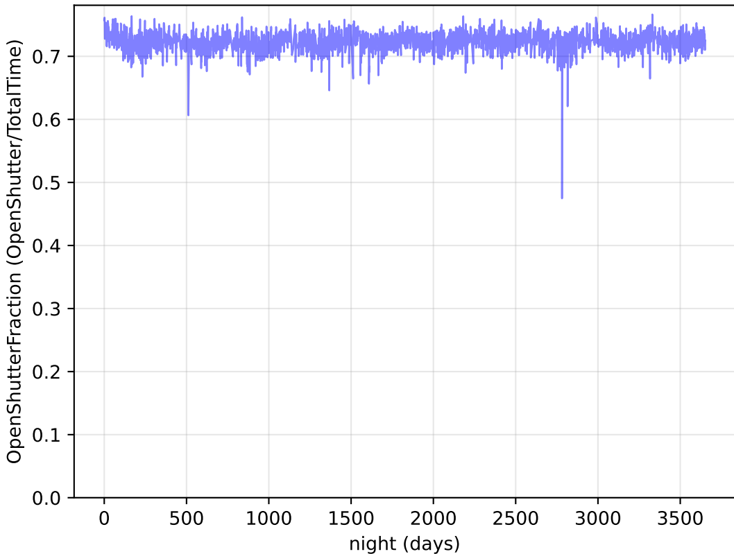
too_elab_r16_d3_giz_v3.4_10yrs : OpenShutterFraction
