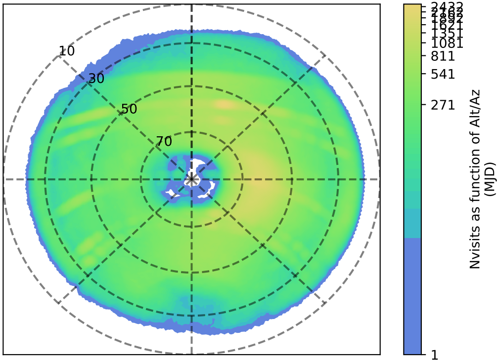
too_elab_r16_d3_giz_v3.4_10yrs z: Nvisits as function of Alt/Az
