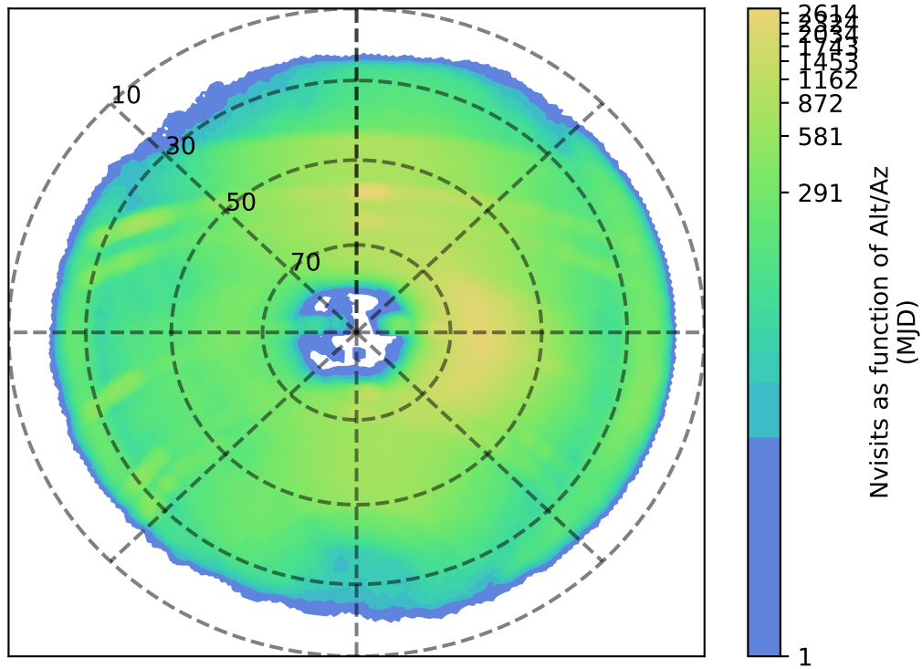
too_elab_r16_d3_giz_v3.4_10yrs i: Nvisits as function of Alt/Az
