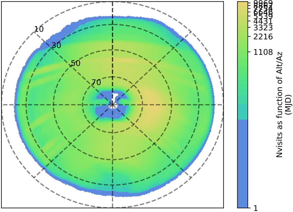
too_elab_r16_d3_giz_v3.4_10yrs : Nvisits as function of Alt/Az
