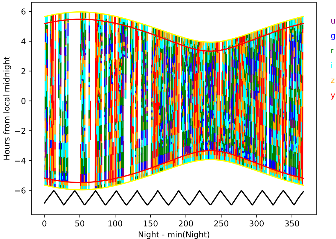
too_elab_r16_d3_giz_v3.4_10yrs year 8-9: Hourglass
