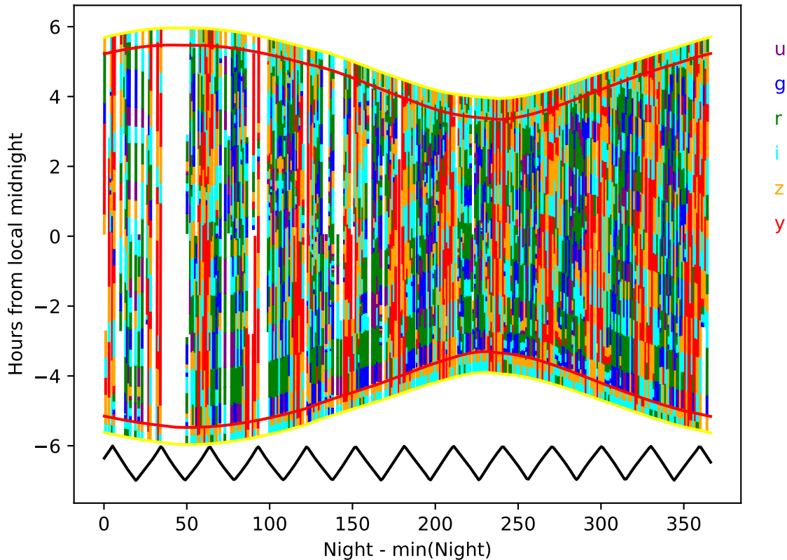
too_elab_r16_d3_giz_v3.4_10yrs year 6-7: Hourglass
