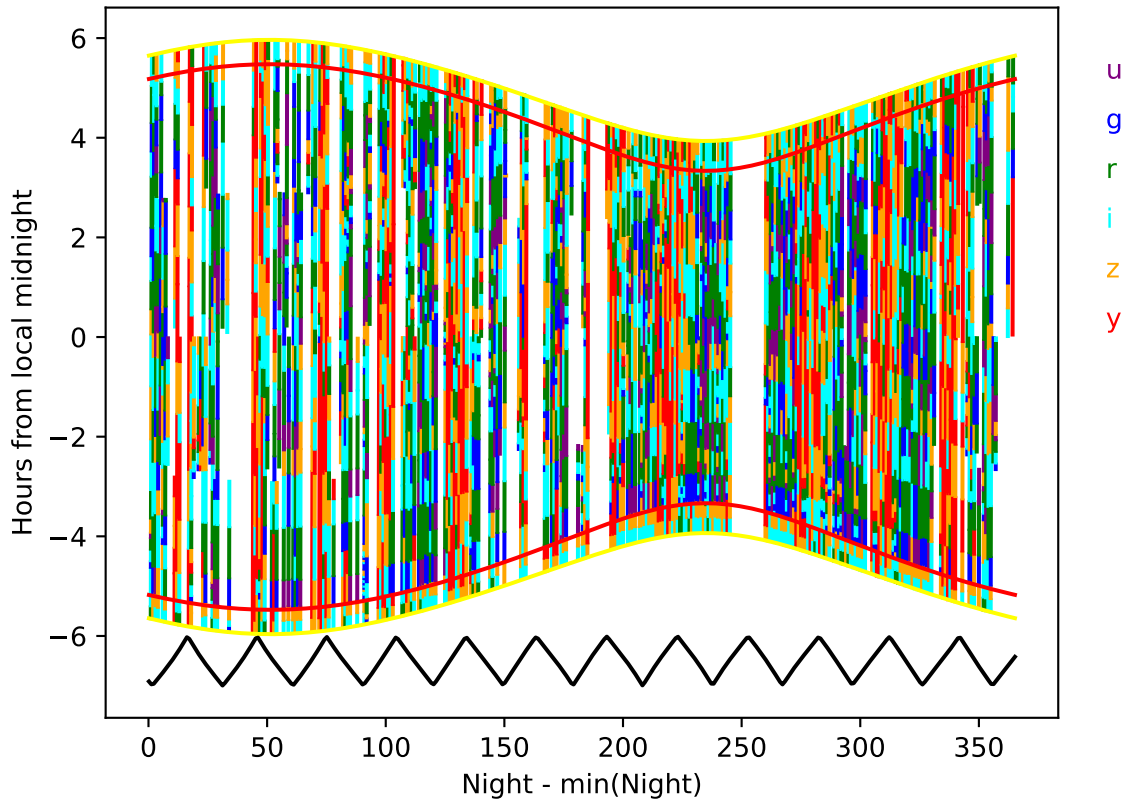
too_elab_r16_d3_giz_v3.4_10yrs year 5-6: Hourglass
