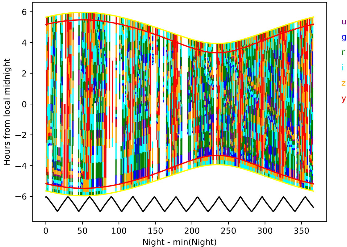
too_elab_r16_d3_giz_v3.4_10yrs year 1-2: Hourglass
