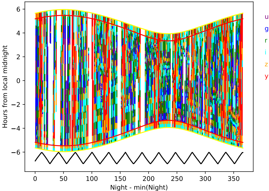
too_elab_r16_d3_giz_v3.4_10yrs year 0-1: Hourglass
